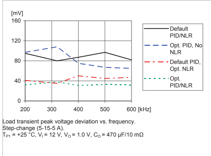
Load transient vs. Switch Frequency
