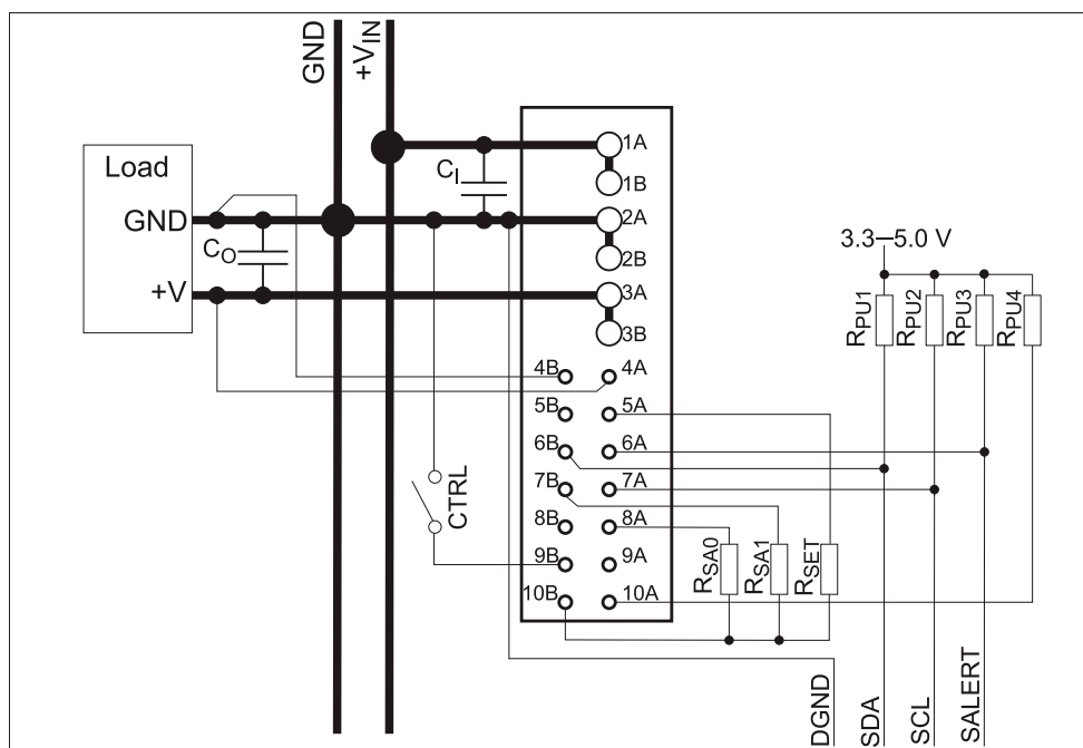
Standalone operation with PMBus communication. Top view of product footprint.
