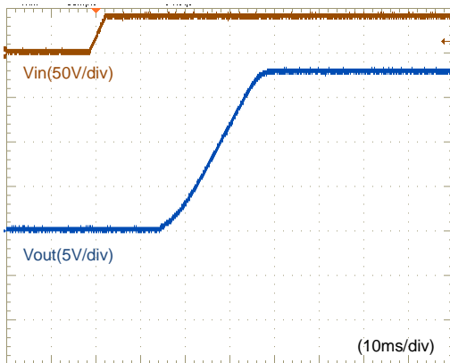
Fig.12-2-13. Start-up Waveform ( I_o=0A )
