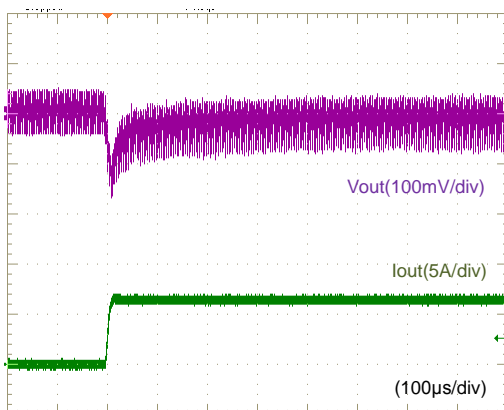
Fig.12-2-17. Load Transient Response ( I_o=0 \rightarrow 6A )
