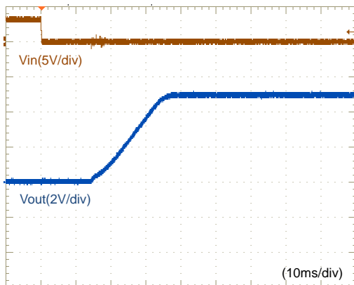
Fig.12-2-3. Start-up Waveform ( I_o=0A )
