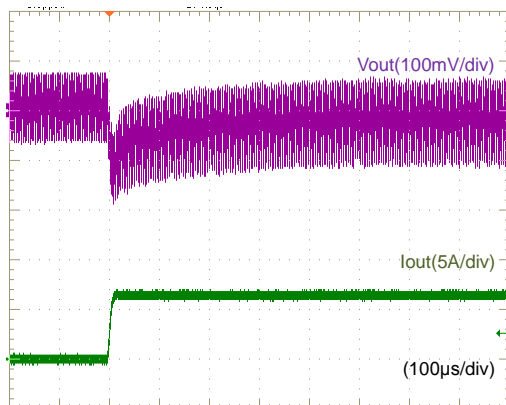
Fig.12-2-23. Load Transient Response ( I_o= 0 \rightarrow 6A )
