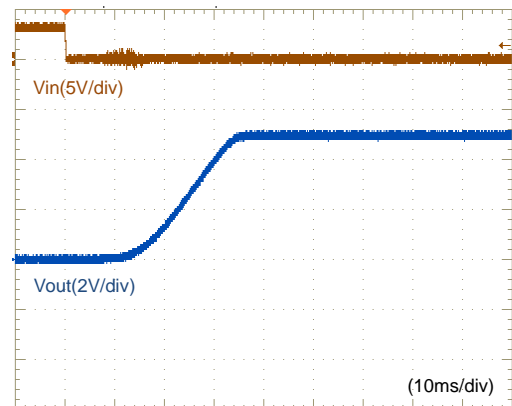
Fig.12-2-4. Start-up Waveform ( I_o=6A )
