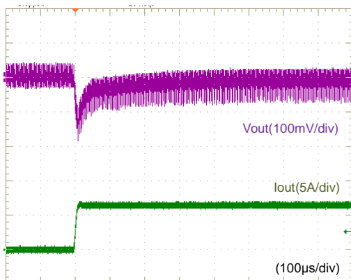
Fig.12-2-5. Load Transient Response ( I_o= 0 \rightarrow 6A )
