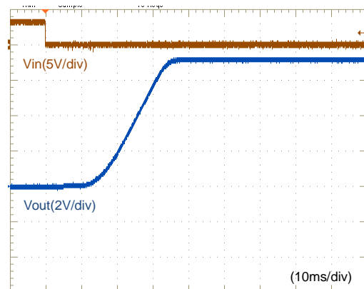
Fig.12-2-22. Start-up Waveform ( I_o=6A )
