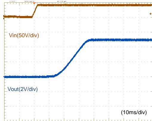
Fig.12-2-8. Start-up Waveform ( I_o=6A )
