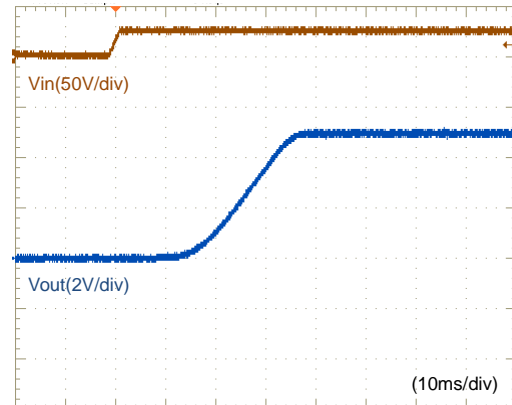
Fig.12-2-2. Start-up Waveform ( I_o=6A )
