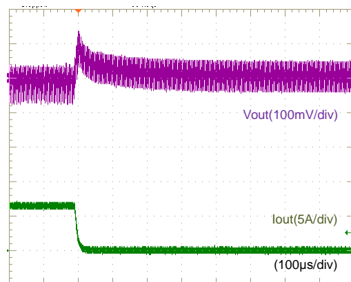
Fig.12-2-18. Load Transient Response ( I_o=6A \rightarrow 0 )
