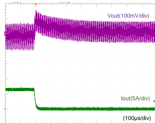
Fig.12-2-24. Load Transient Response ( I_o= 6A \rightarrow 0 )
