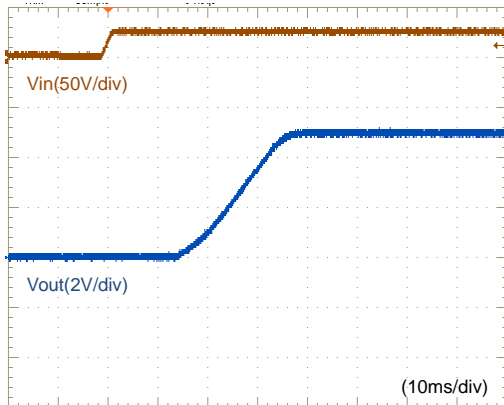
Fig.12-2-1. Start-up Waveform ( I_o=0A )
