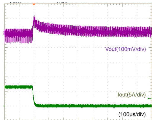
Fig.12-2-6. Load Transient Response ( I_o= 6A \rightarrow 0 )
