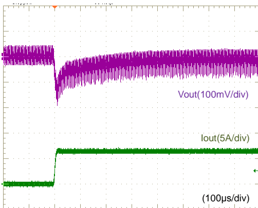
Fig.12-2-11. Load Transient Response ( I_o= 0 \rightarrow 6A )
