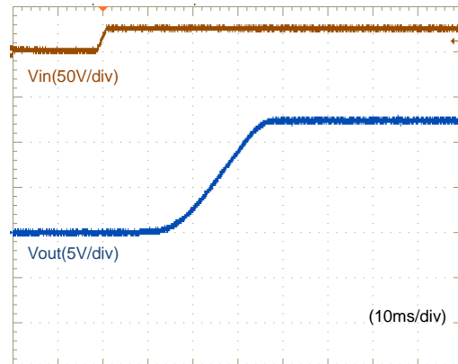
Fig.12-2-20. Start-up Waveform ( I_o=6A )
