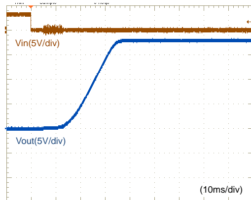
Fig.12-2-16. Start-up Waveform ( I_o=6A )
