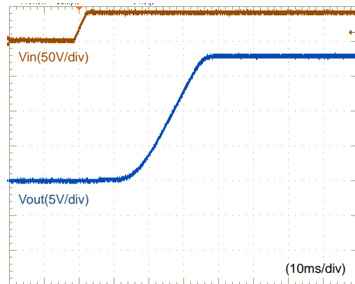
Fig.12-2-14. Start-up Waveform ( I_o=6A )
