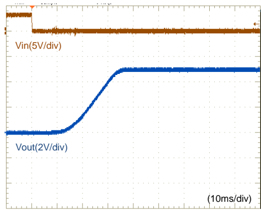
Fig.12-2-10. Start-up Waveform ( I_o=6A )
