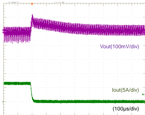
Fig.12-2-12. Load Transient Response ( I_o= 6A \rightarrow 0 )
