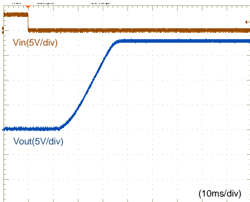
Fig.12-2-15. Start-up Waveform ( I_o=0A )
