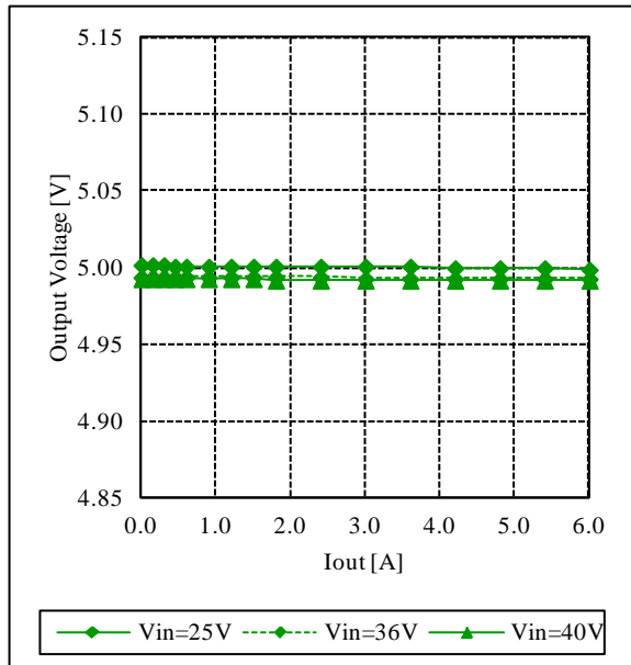
Fig.12-1-1. Output Voltage vs. Output Current
