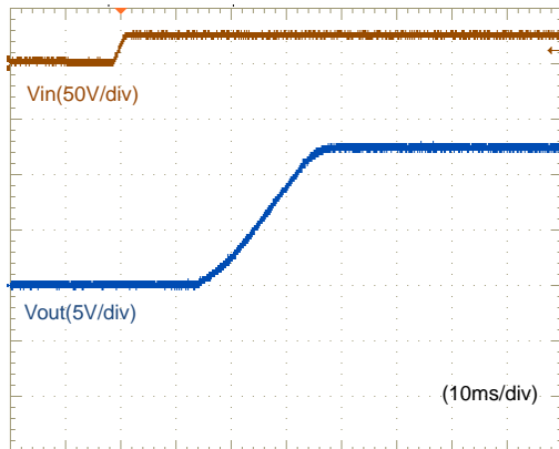
Fig.12-2-19. Start-up Waveform ( I_o=0A )
