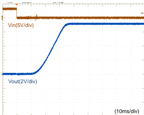
Fig.12-2-21. Start-up Waveform ( I_o=0A )
