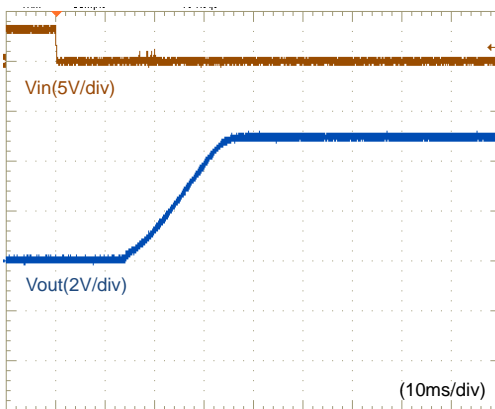
Fig.12-2-9. Start-up Waveform ( I_o=0A )
