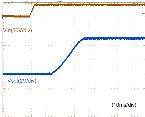
Fig.12-2-7. Start-up Waveform ( I_o=0A )
