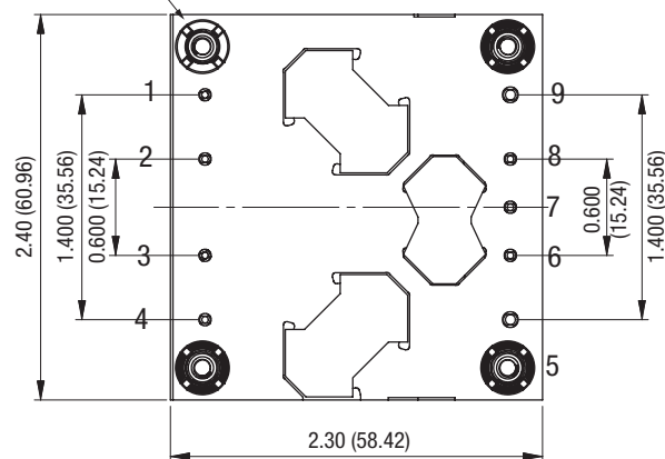
Bottom Pin Side View
