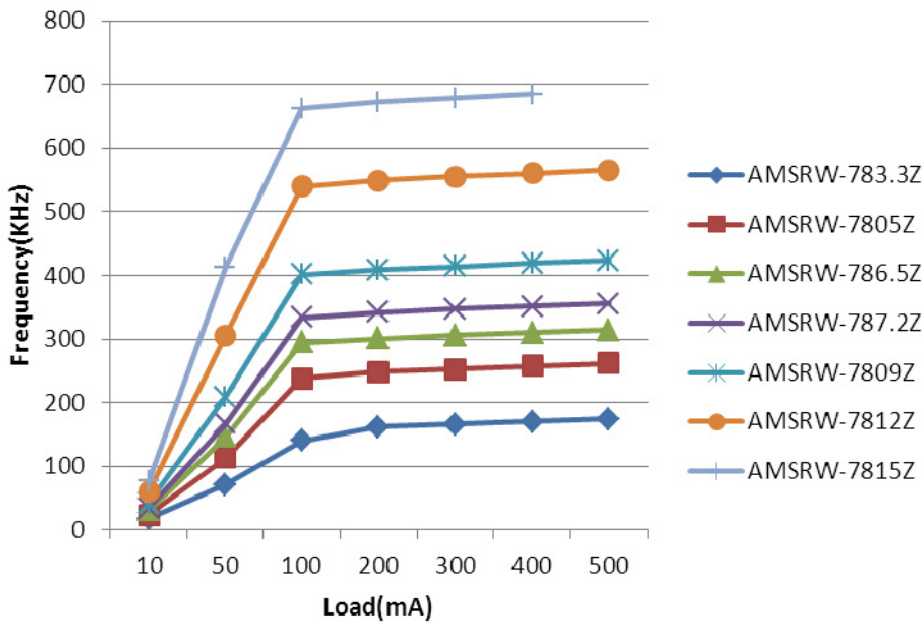
Switching Frequency(KHz) vs. Load(mA) V in = 24V-72V
