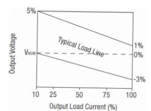
3.3V in, 3V out type only
