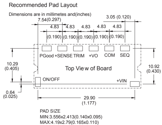
Figure 9. Recommended VPOL16A-12W-SMT Footprint
